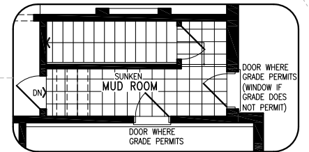
OPT. SERVICE STAIRCASE ELEVATION A
